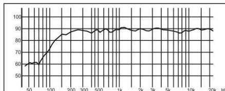
DSP455II Freq.Response (dB SPL, 1W, 1m)
